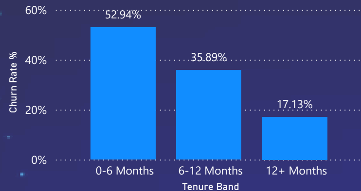
Churn Rate % by Tenure Band
