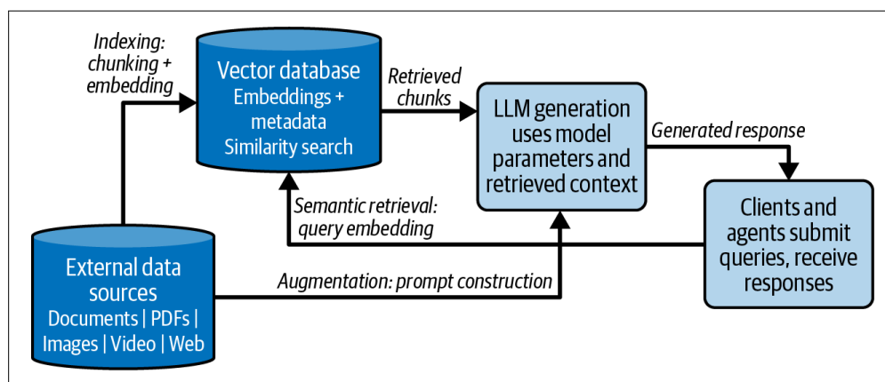
Figure 3-3. Dataflow in RAG apps
