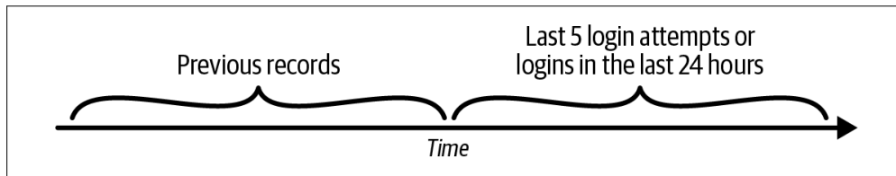
Figure 3-1. An example sliding window context
