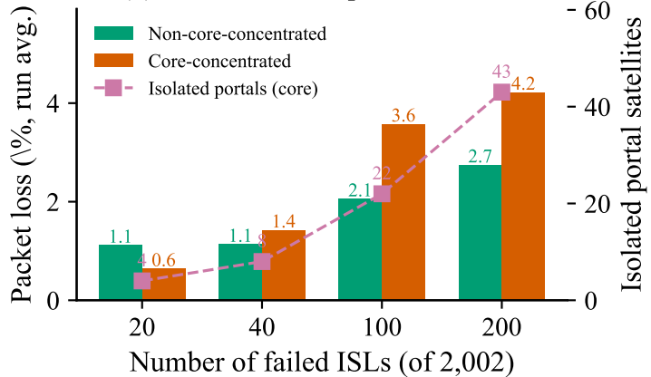
(b) Packet loss and portal isolation
