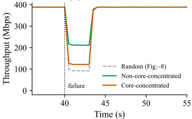
(a) Throughput around failure (200 ISLs)
