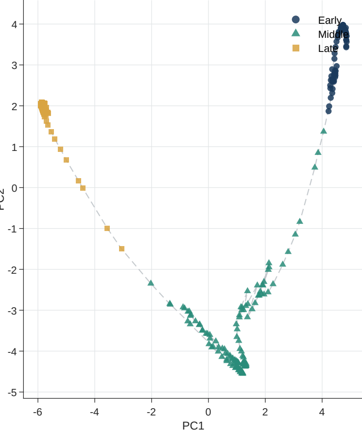
(a) Shared latent PCA, colored + shaped by true stage
