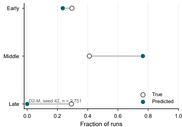
(d) D2-M failure boundary: predicted middle-stage collapse
