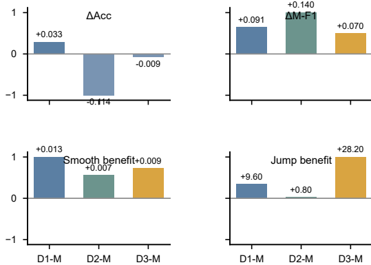
(c) DC-PSR relative gains across cross-machine tasks
