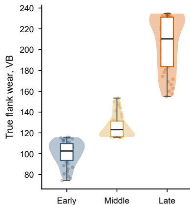
(e) Physical wear semantics by predicted stage
