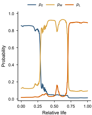
(a) Stage-aware probability evolution along tool life
