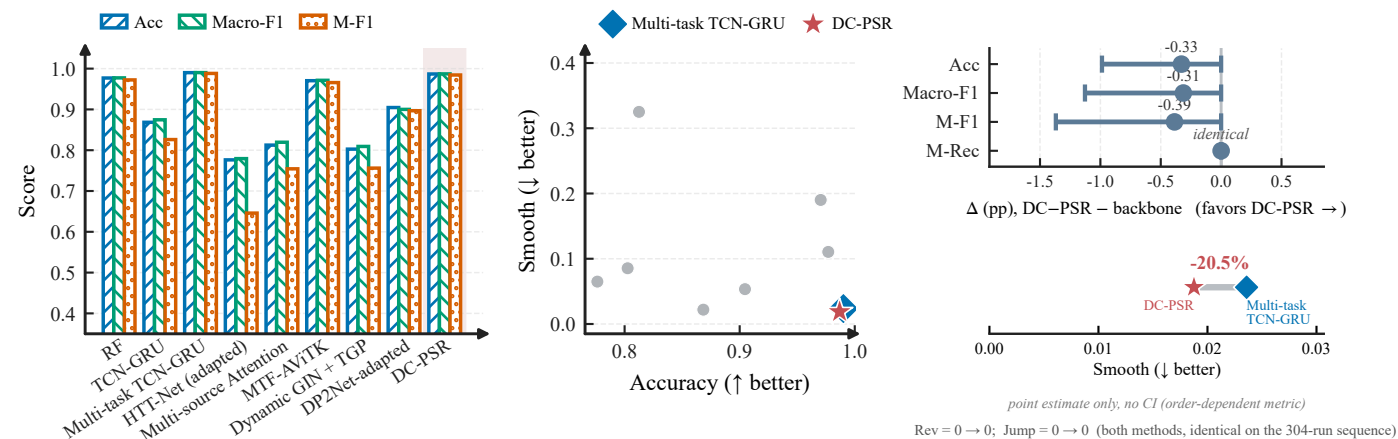
(a) Overall classification performance, 9 methods
