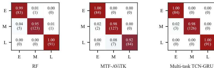
(d) Representative confusion matrices (row-normalized; count)
