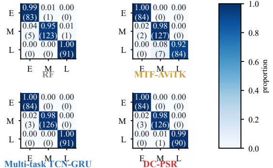
(b) Representative confusion matrices (rows=true, cols=predicted; row-normalized)
