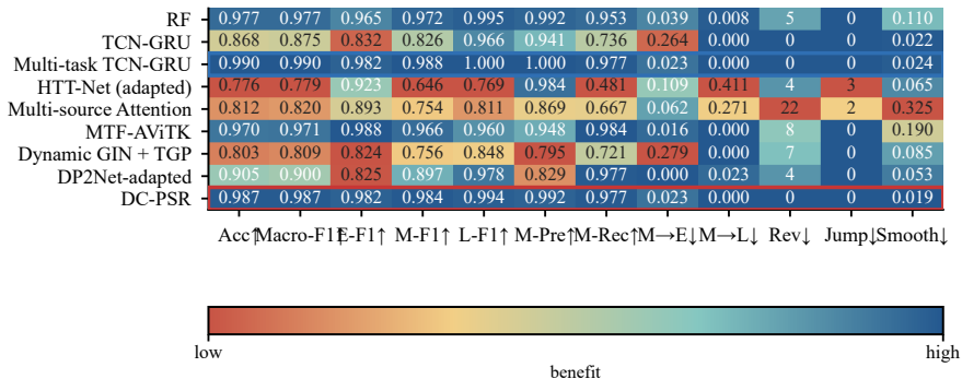
(a) 9-method × metric performance landscape on PHM2010 D1 (n=304)
