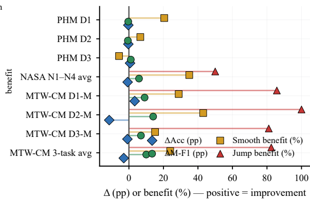
(b) Multi-task TCN-GRU \rightarrow DC-PSR paired gain, PHM/NASA/MTW-CM (Smooth/Jump = benefit = backbone - DC-PSR; positive = improvement)
