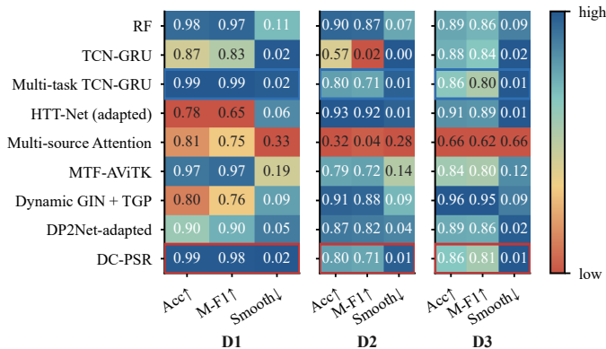
(a) Within-task robustness, PHM2010 D1/D2/D3 \times 9 methods (color = within-task benefit; numbers = raw values)
