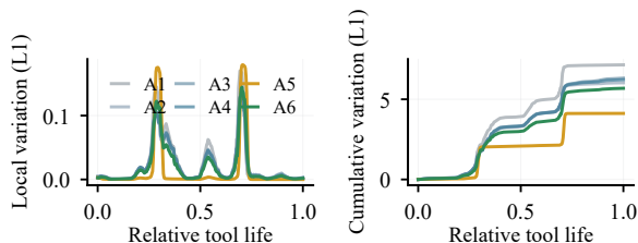
(d) Lifecycle probability variation (local + cumulative); Rev=Jump=0 for all A1–A6 (real)
