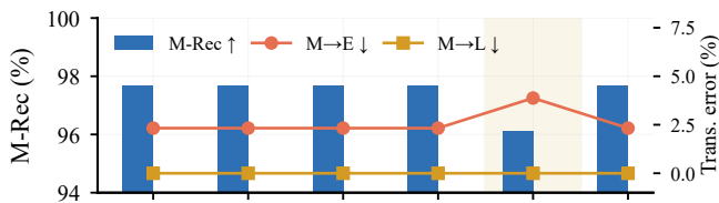
(c) Middle-stage recall & transition error: classification largely unchanged A1–A4 despite shifting probability geometry
