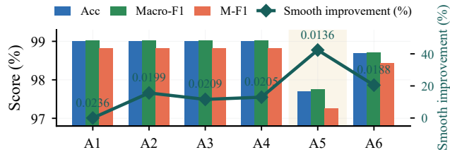
(a) Predictive performance across A1→A6 (Smooth shown as improvement vs A1, %)
