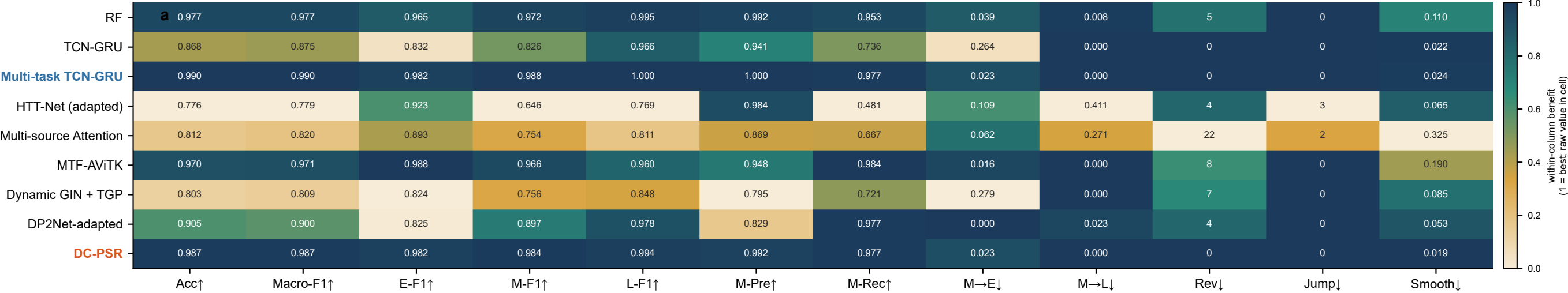
9-method × metric performance landscape on PHM2010 D1 (n=304)
