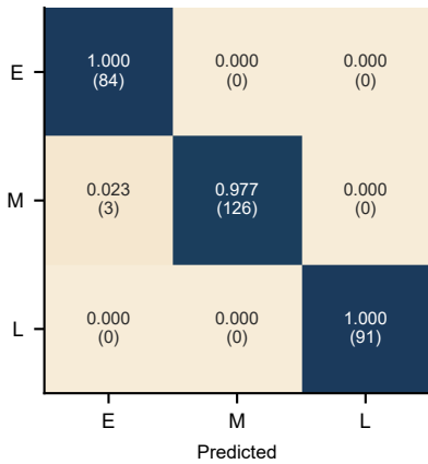
Multi-task TCN-GRU
