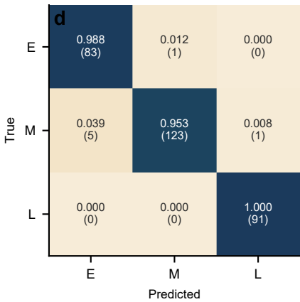
RF
