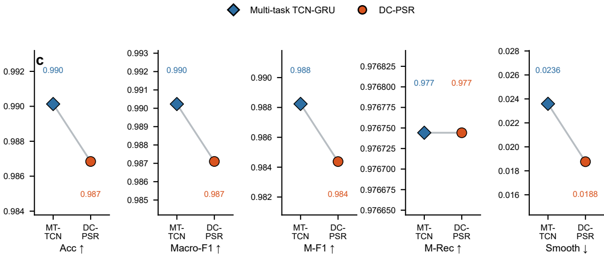
Controlled comparison: DC-PSR vs. its Multi-task TCN-GRU backbone
