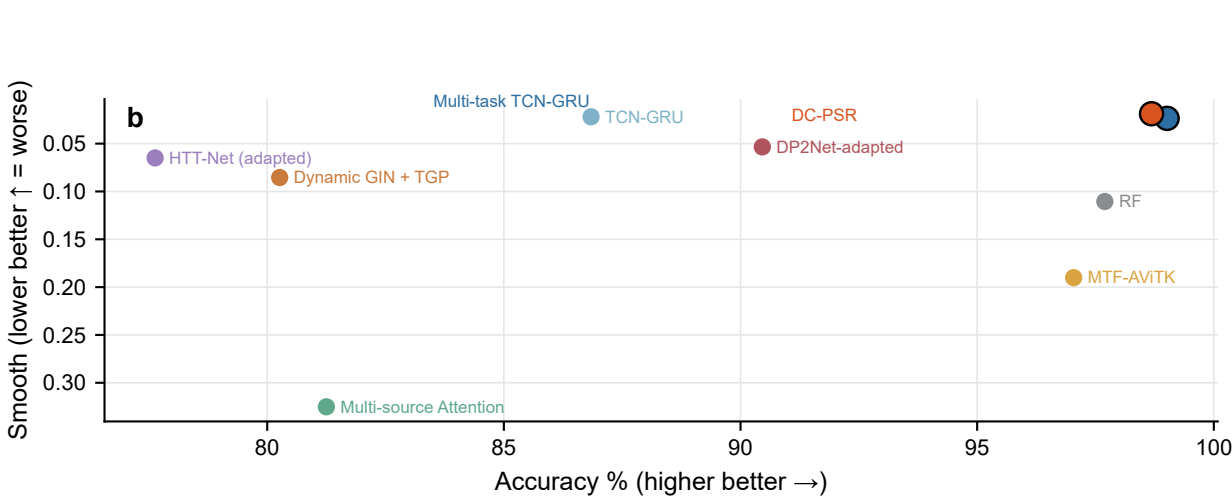
Accuracy–consistency trade-off (dashed = non-dominated frontier)
