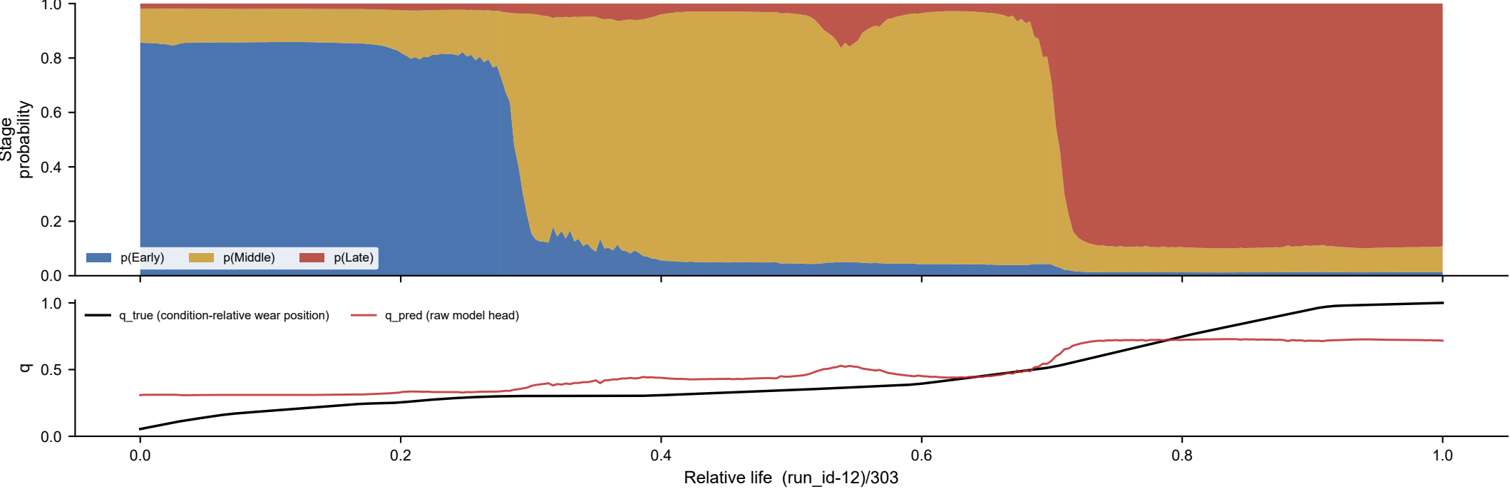
(a) Full C6 lifecycle: stage probability + degradation position (n=304)
