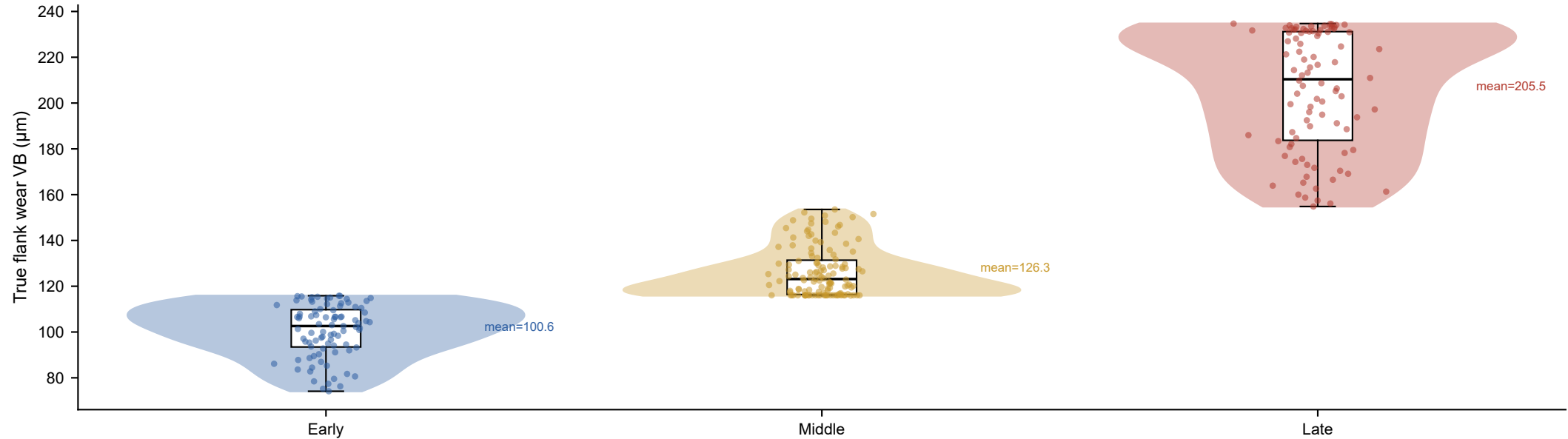
(d) Physical wear anchor: VB_true grouped by predicted stage
