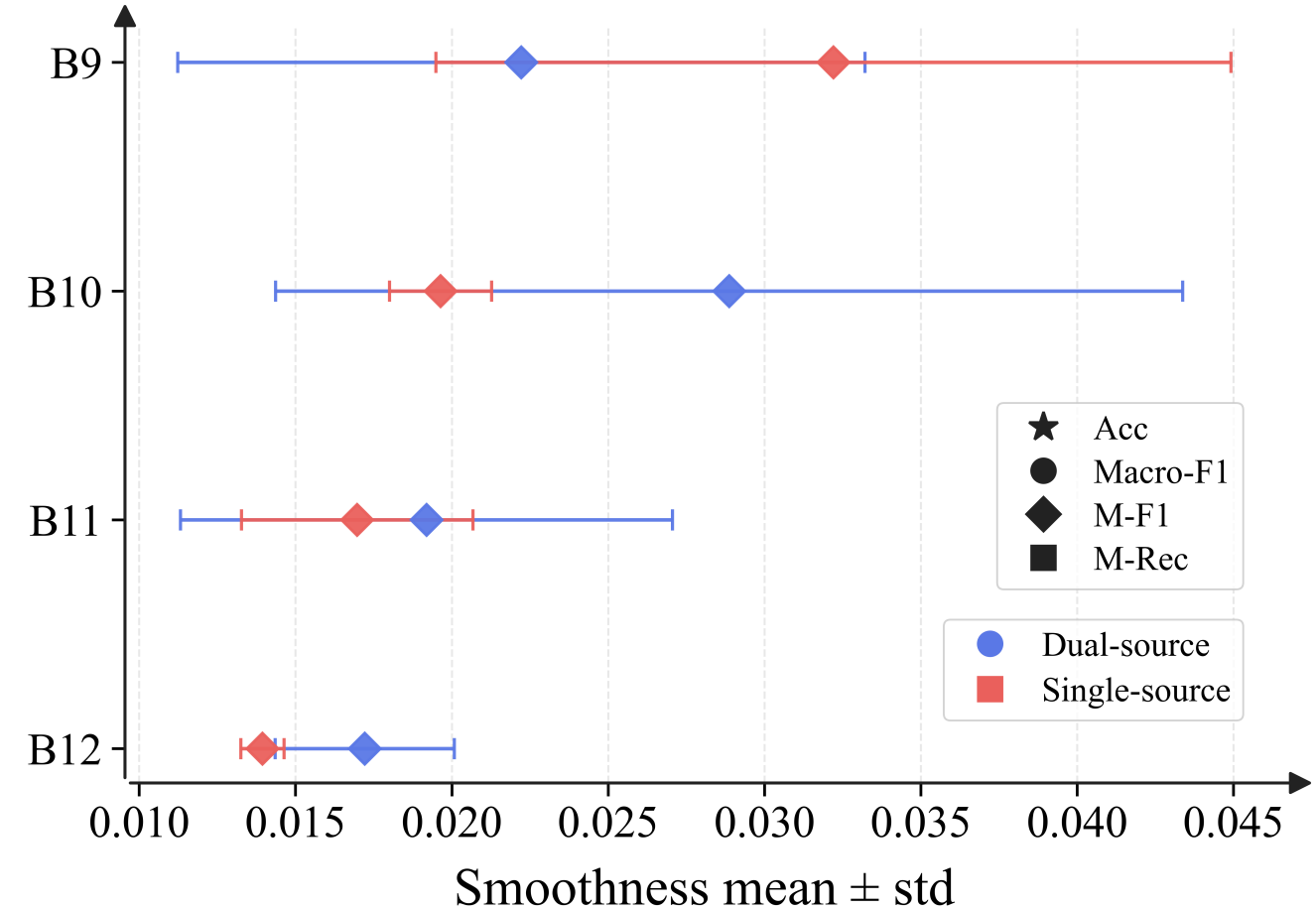
(b) Probability smoothness
