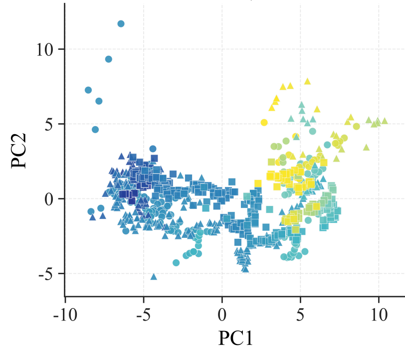
(b) Raw features / q_{c,t}
