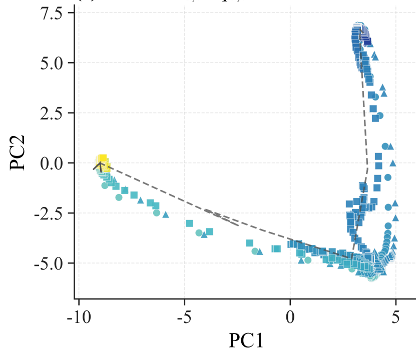
(e) Shared h_{c,t} / q_{c,t}
