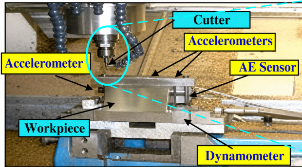
High Speed Milling Machine
