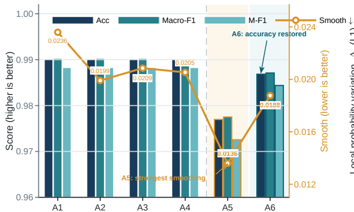
(a) Overall predictive performance across A1 - A6
