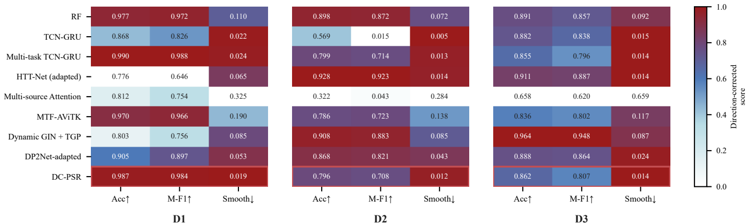
(a) Task-level 9-method landscape (D1/D2/D3; color = direction-corrected score, cell = raw value)
