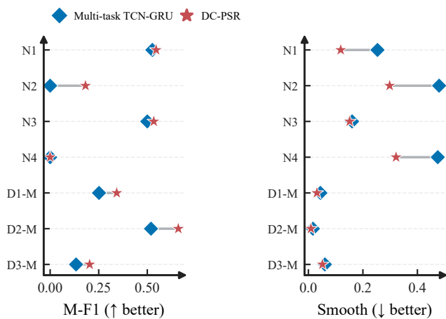
(c1) M-F1 by task (NASA + MTW-CM)
