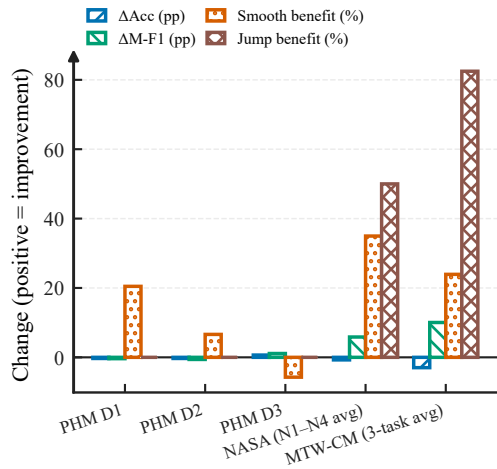
(b) Backbone \rightarrow DC-PSR paired change across conditions/datasets
