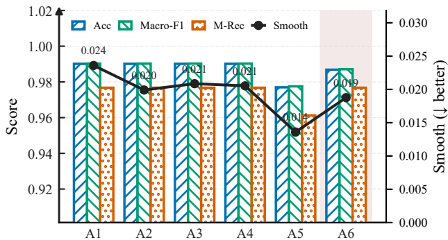
(a) Hard-decision performance & Smooth, A1→A6
