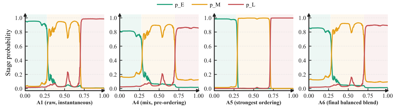
(c) Probability-state formation: p_E / p_M / p_L over the C6 lifecycle, representative configurations
