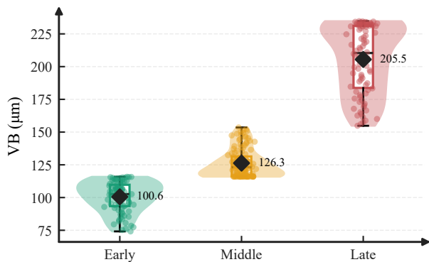
(e2) Physical wear (VB) by predicted stage
