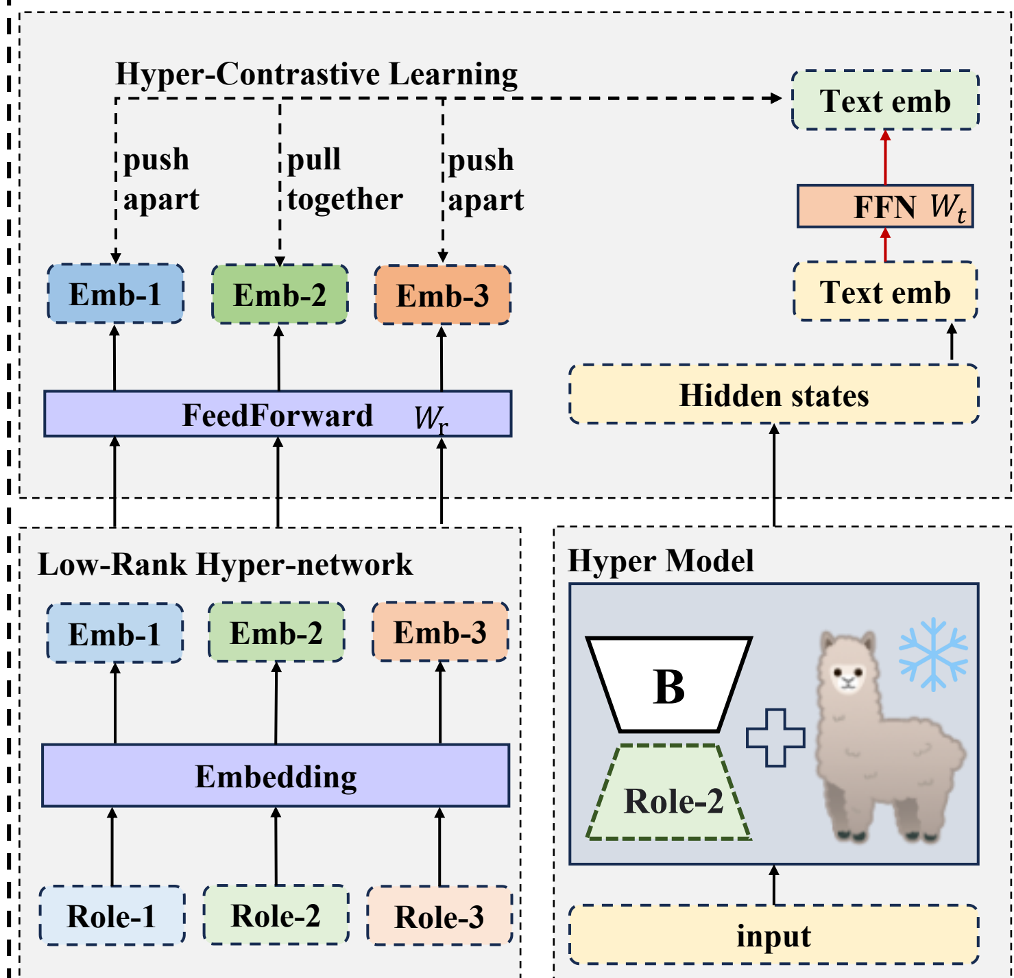
(b) Hyper-Contrastive Learning
