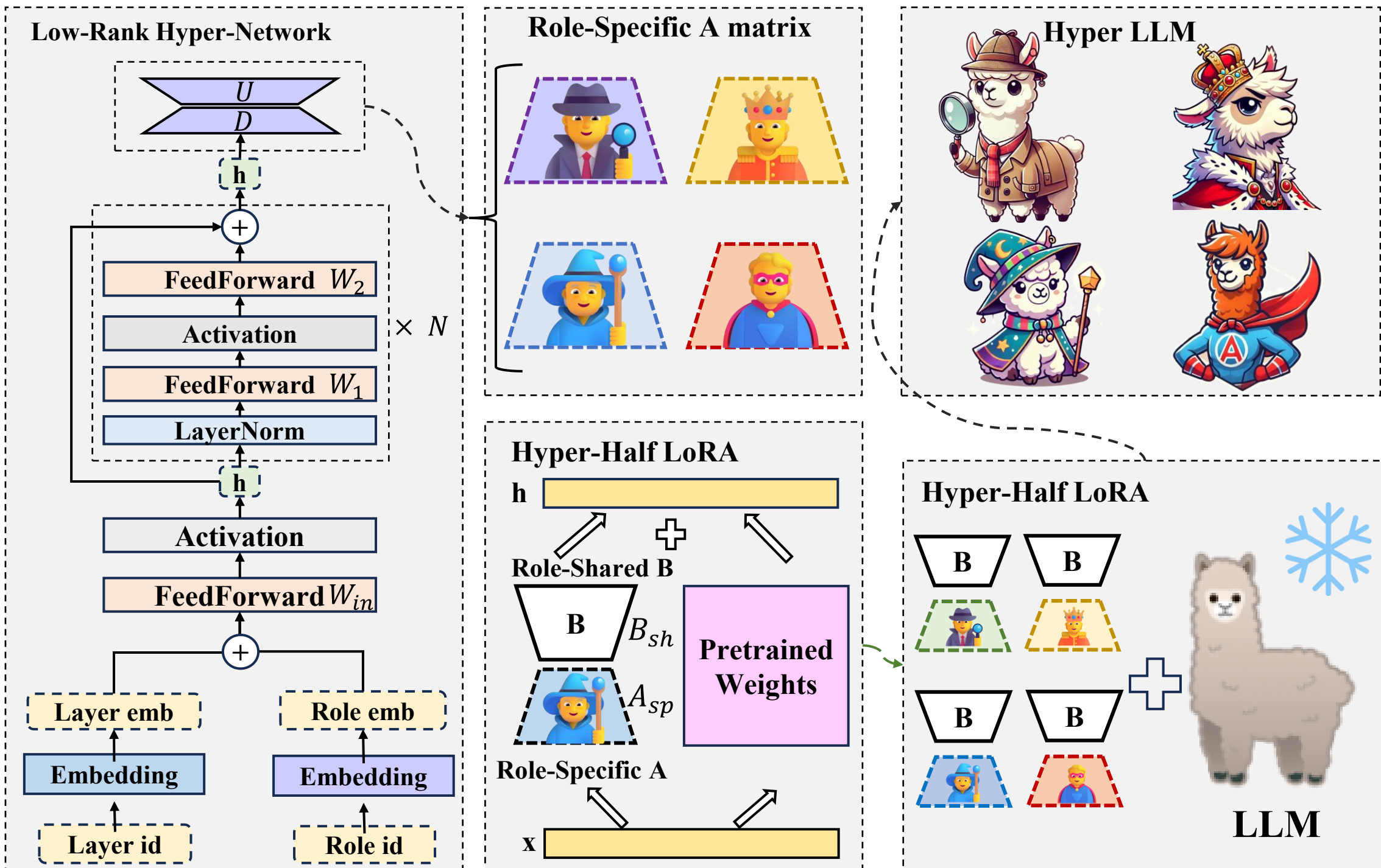
(a) Hyper-Half LoRA structure
