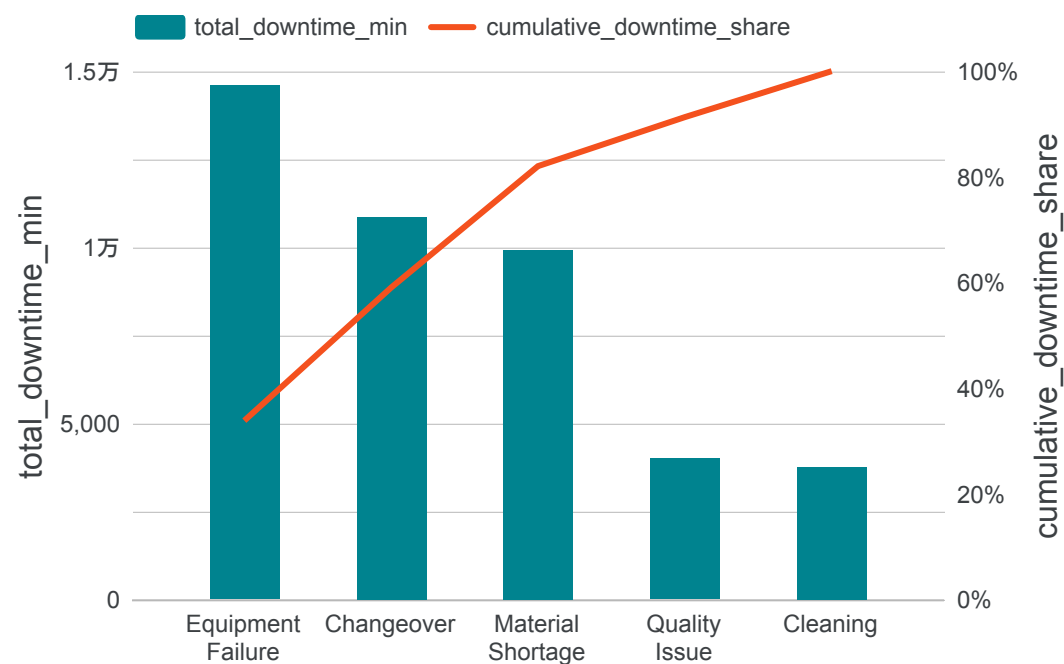
Downtime Reason Pareto
