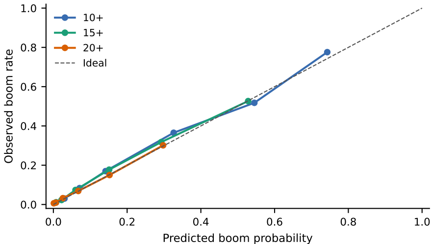
Probability calibration
