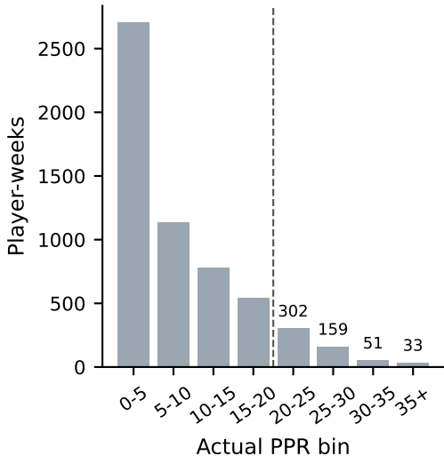
2024 score distribution
