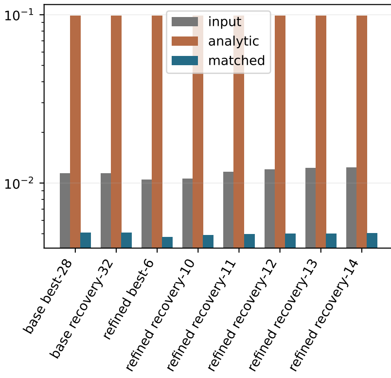
A RMSE
