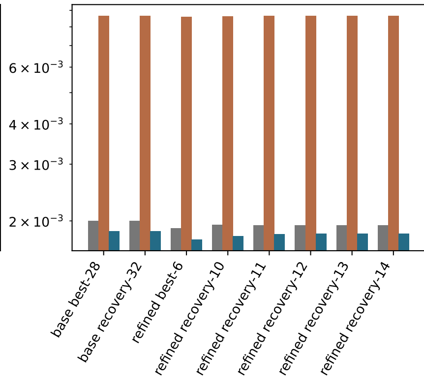
C RMSE
