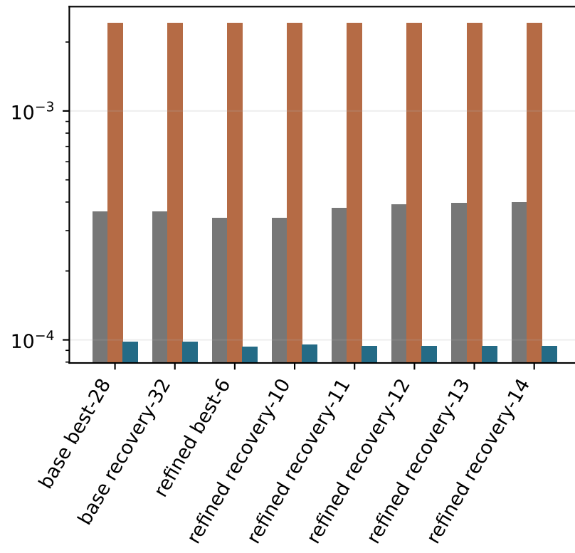
B RMSE
