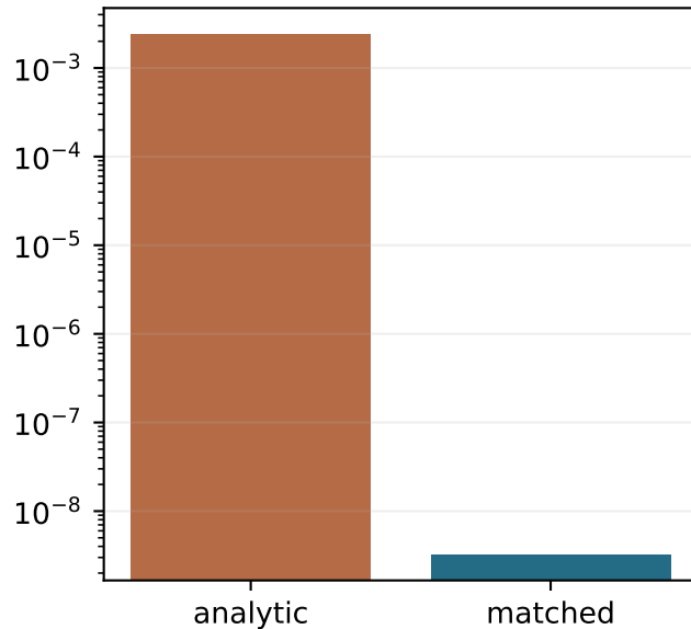
B RMSE
