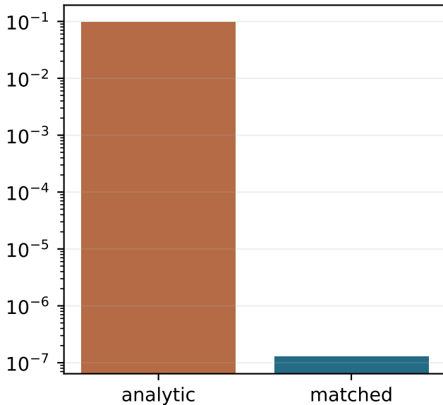
A RMSE
