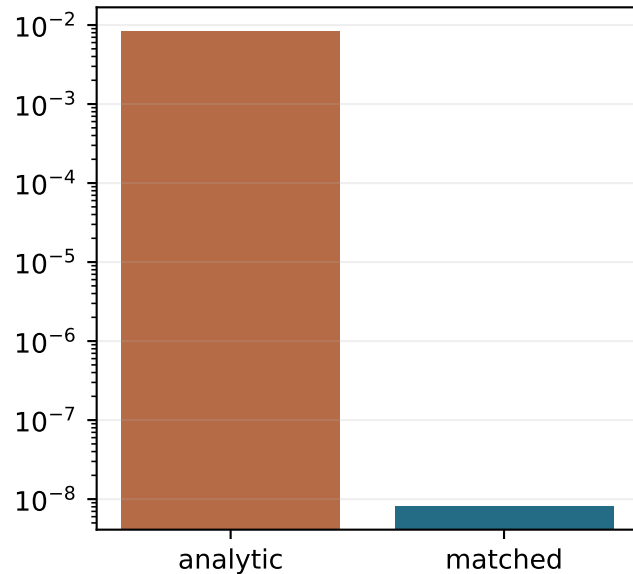
C RMSE
