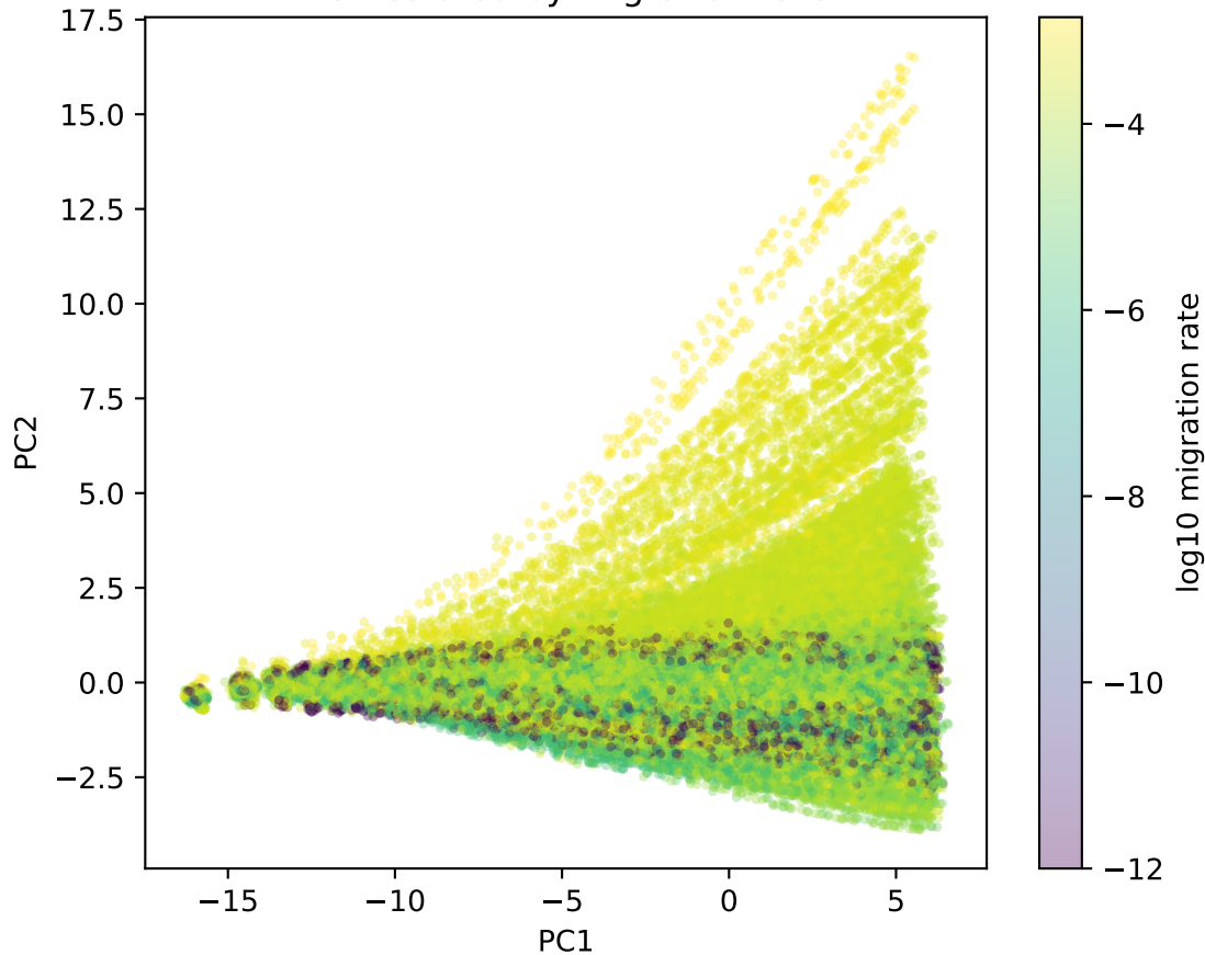
PCA colored by migration rate
