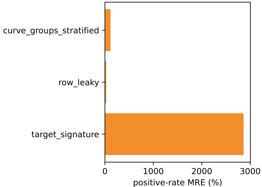
Regression
