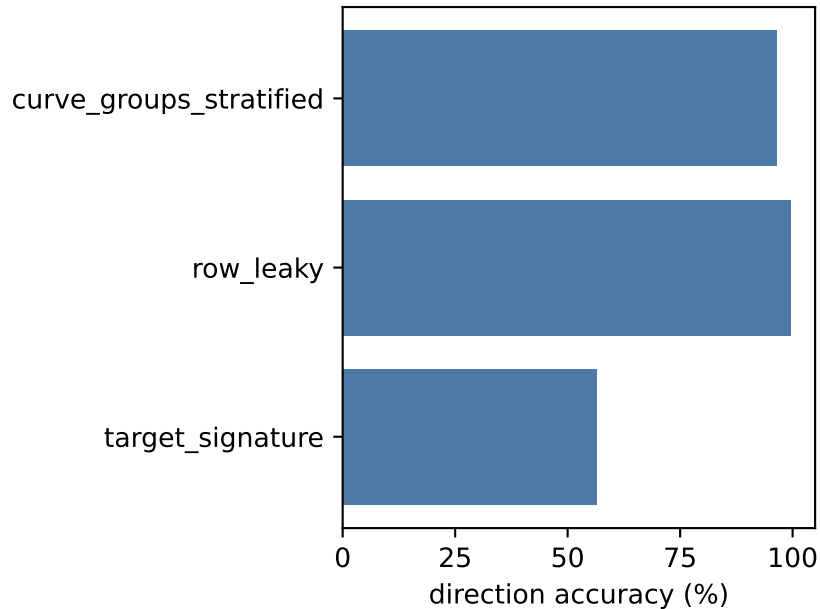
Classification
