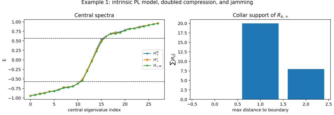
Figure 4: Central spectra of H_+^{\text{PL}}(\mathcal{K}) , H_+^{\partial}(\mathcal{K}) , and H_{+,M} on the disk-like example, together with the measured support distribution of the collar correction R_{\partial,+} . The correction is not norm-small, but it is boundary-collar supported, as predicted by Theorem 2.8.
