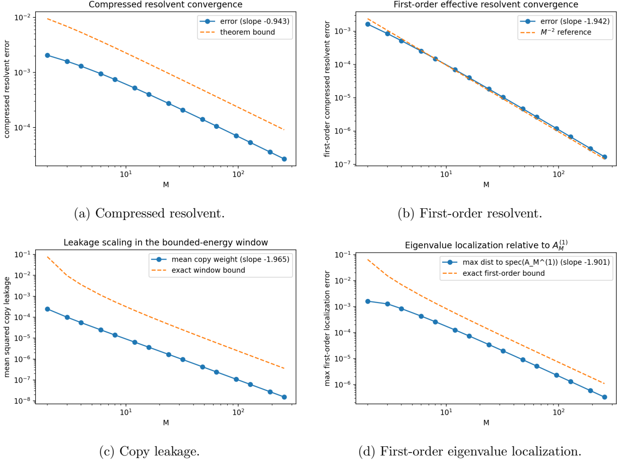
Figure 5: Log-log finite- M checks. The compressed resolvent slope tracks the M^{-1} rate of Theorem 3.2; the first-order resolvent, squared copy leakage, and first-order eigenvalue localization track the M^{-2} rates of Theorems 3.5 and 3.10 and the first-order eigenvalue localization theorem stated in the supplement (Section 7.32). Fitted slopes and additional rate diagnostics are reported in the supplement, Section 10.
