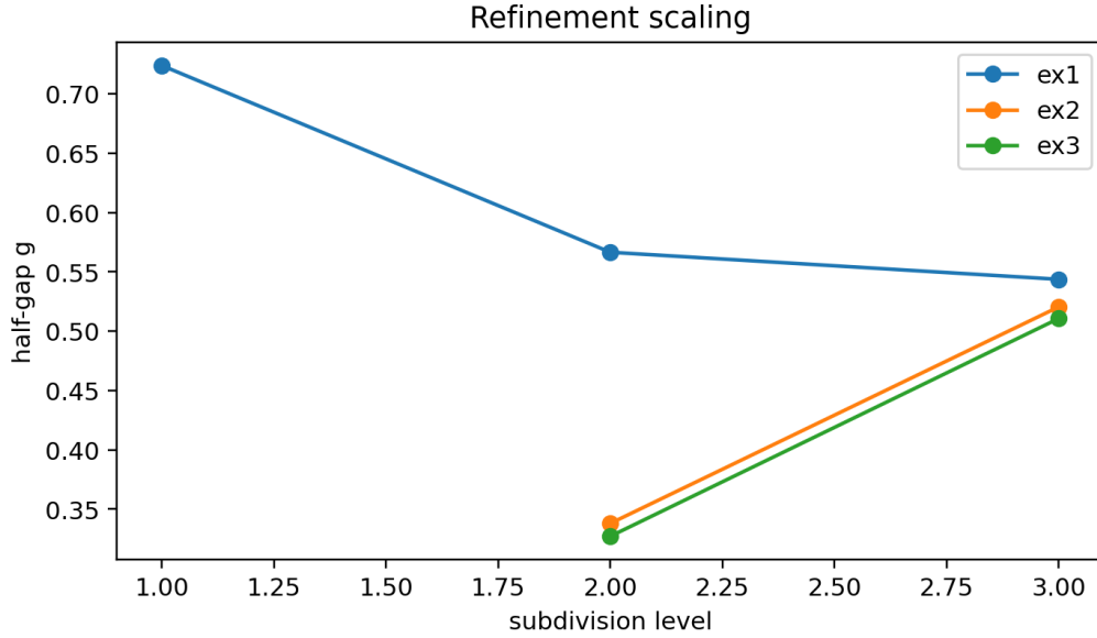
Figure 14: Measured bulk half-gap g_{\text{gap}} versus subdivision level for the three example families. This finite-mesh check documents the sampled matrices; theorem-level gap input comes from HP or from the periodic proof.
