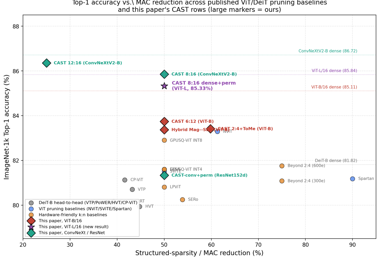
Figure 4: Post-FT top-1 vs. reported sparse-execution MAC reduction. Points are rows from Table 6; marker size distinguishes this paper’s CAST rows, color encodes architecture family, and dotted lines mark dense timm baselines. MAC reduction is computed against each cited method’s own dense baseline.
