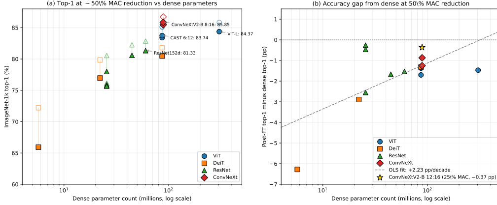
Figure 3: \Delta Top-1 relative to dense at approximately 50% sparse-execution MAC reduction vs. dense parameter count. Points are rows of Table 5; the dashed line is an OLS fit in \log_{10} parameters.
