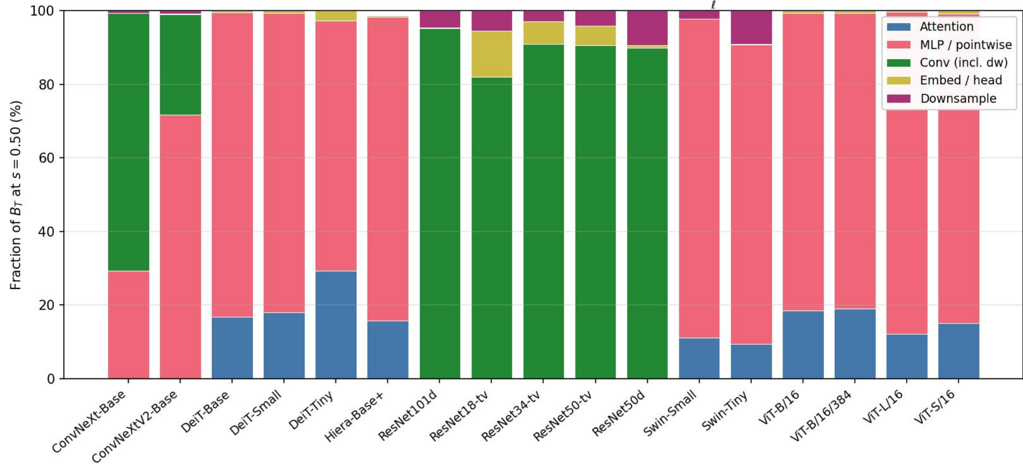
Theorem~5.13: per-architecture concentration of the data-path budget \sum_{\ell} B_{T,\ell} at s = 0.50 , by layer type
