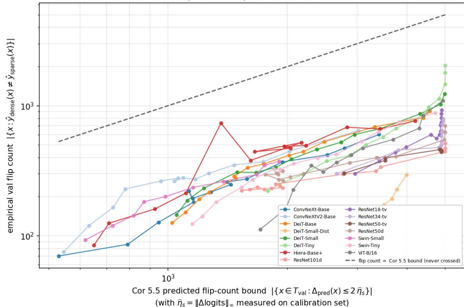
Val-side verification of Corollary 5.5: 195 cycles across 15 architectures, 0/195 violations
