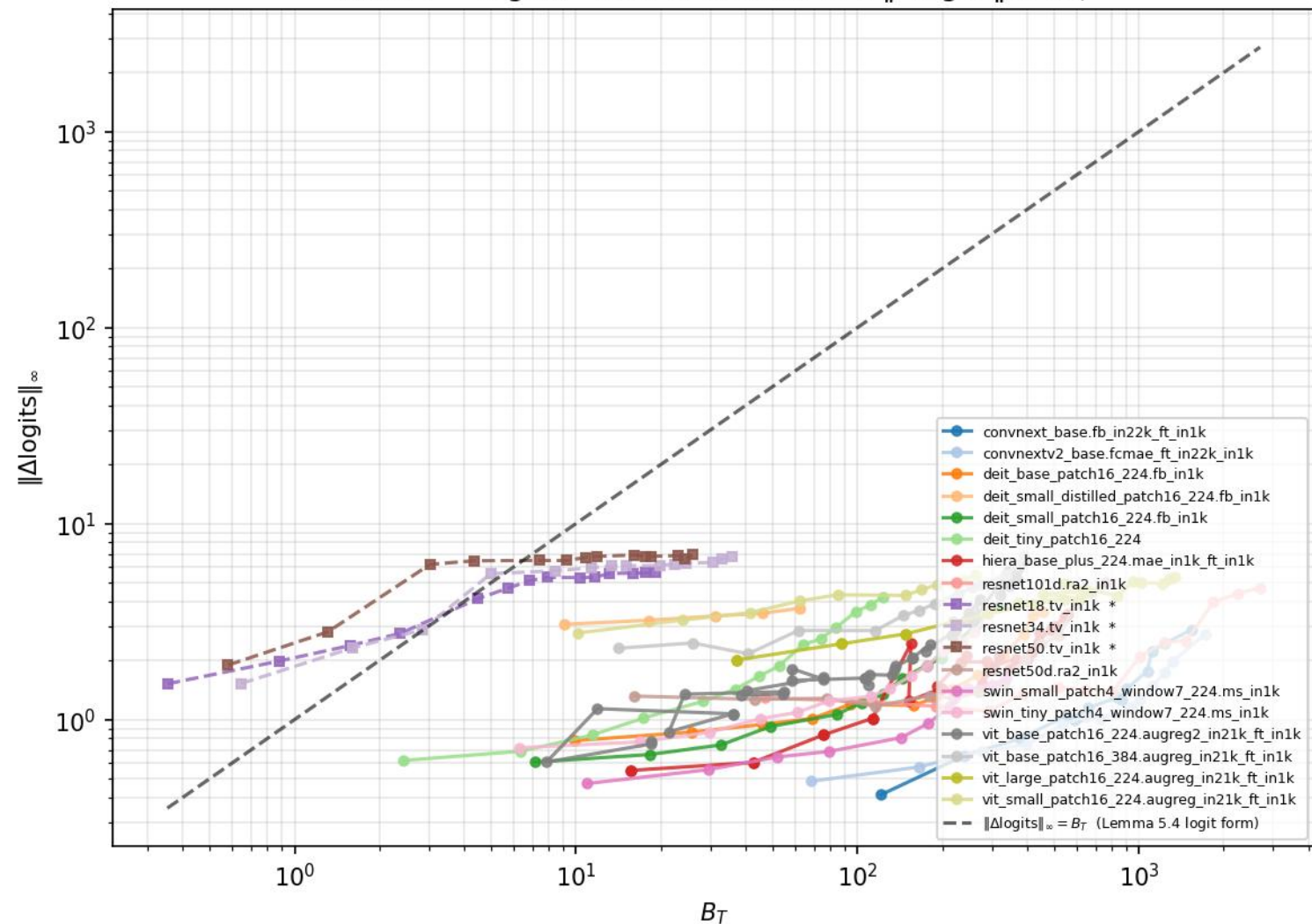
Audit 4 — logit- \ell^\infty form of Lemma 5.4: \|\Delta\text{logits}\|_\infty \leq B_T
