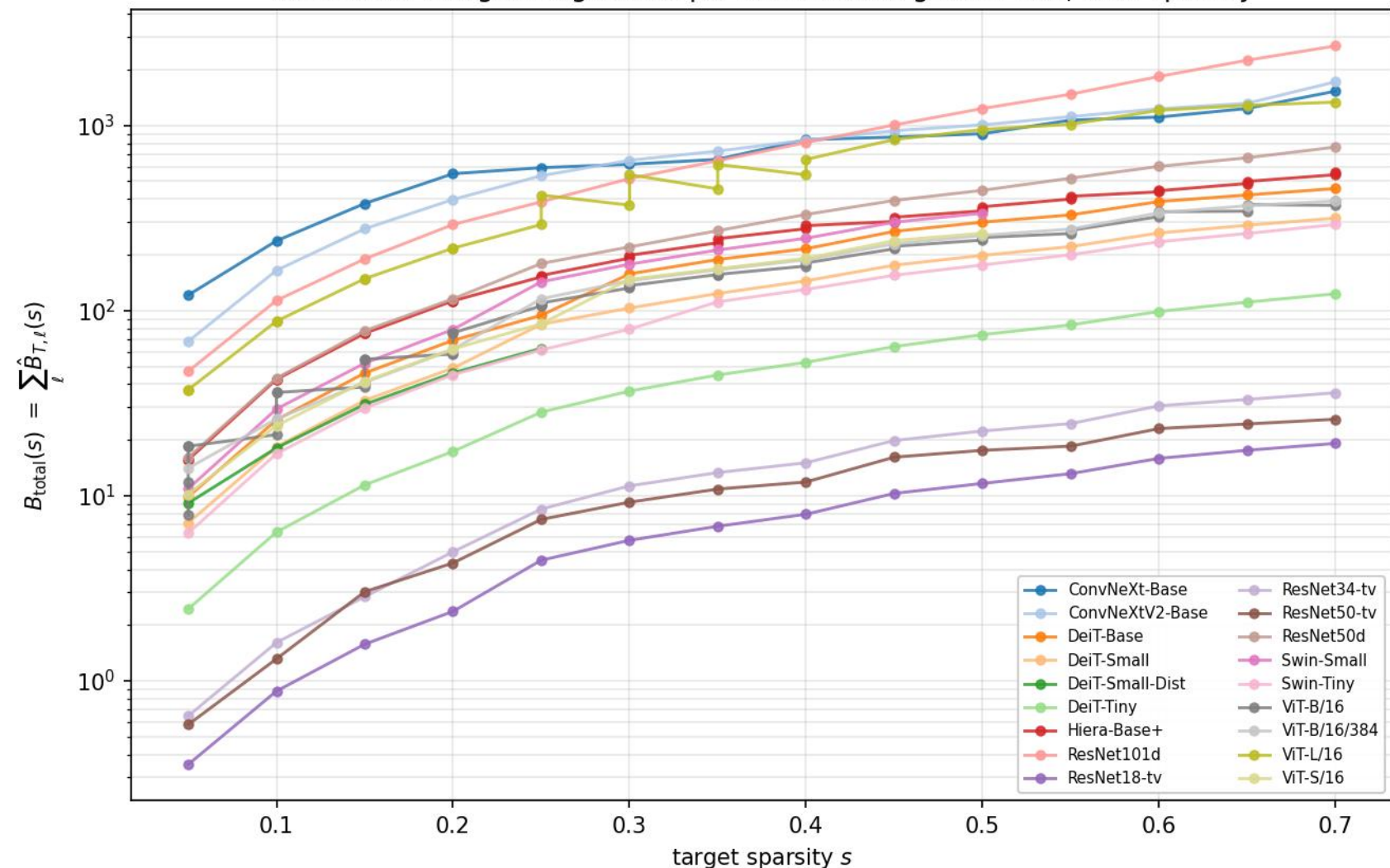
Lemma 5.4 budget magnitude: per-architecture growth of B_T with sparsity
