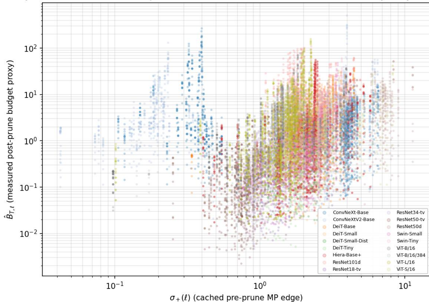
Corollary 5.14 universal scatter — pooled Pearson r = +0.241 on n = 19227 (arch, layer, cycle) data points
