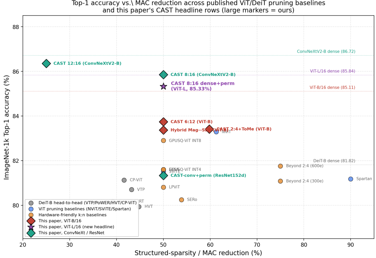
Figure 4: Post-FT Top-1 accuracy vs. structured-sparsity / MAC reduction across published ViT/DeiT pruning baselines and this paper’s CAST headline rows (large markers). Baselines (grey/blue/orange dots) are the rows of Table 6; our rows are coloured by architecture family (red = ViT-B/16, purple star = ViT-L/16, teal = ConvNeXt/ResNet). Dotted horizontal lines mark the dense timm baselines for each architecture family. The CAST 8:16 dense+perm on ViT-L/16 row (purple star, 85.33%) is within 0.51 pp of its dense baseline at 50% structured sparsity, the smallest dense-gap of any plain-ViT-family row in this paper. Among the DeiT-Base baselines plotted, a few (NViT -0.07 pp at \sim 61\% MAC; Beyond 2:4 at 600 training epochs -0.08 pp; ELSA -0.20 pp) close the dense-gap further on the smaller DeiT-B architecture, but all use 50–600 fine-tuning epochs vs. our 3-epoch budget. The figure uses \text{MAC-reduction} = 1 - \text{FLOPs}_{\text{post}} / \text{FLOPs}_{\text{dense}} on the cited paper’s own dense baseline (e.g. NViT 1 - 6.8 / 17.56 = 61.3\% ; Beyond 2:4 V:N:M 64:2:8 = 75\% pattern sparsity).
