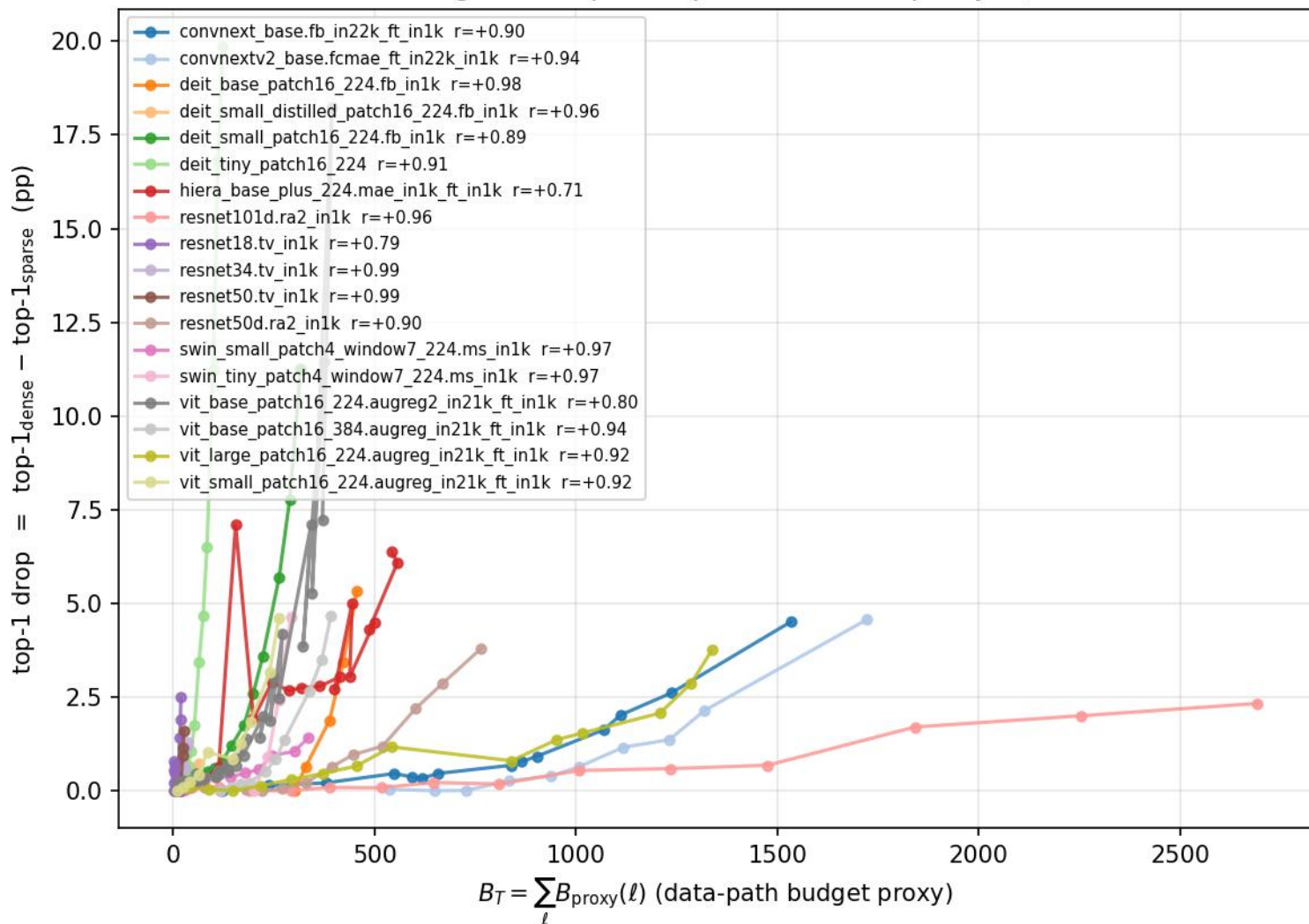
Bridge 1 — top-1 drop vs certificate proxy B_T
