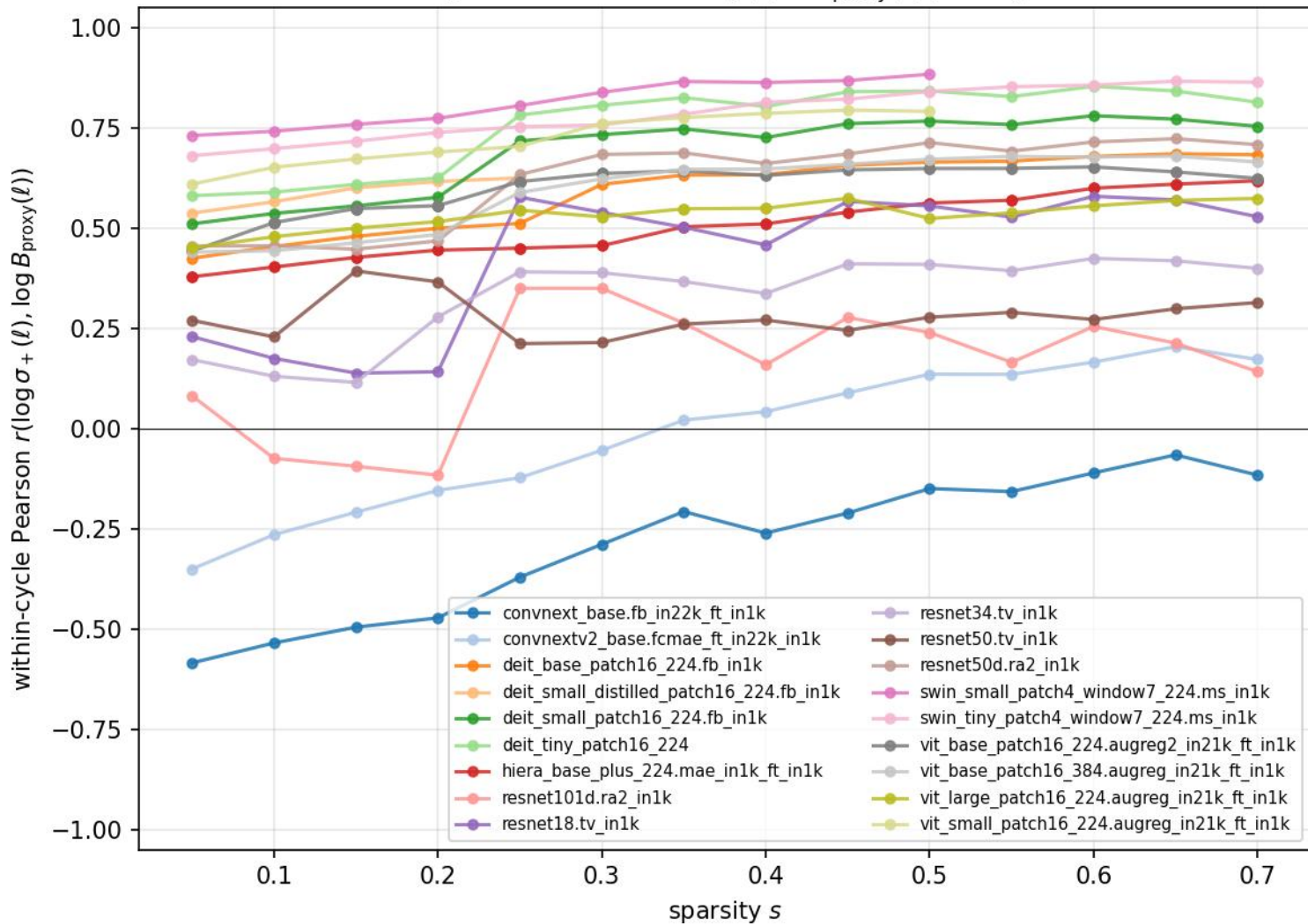
Bridge 3 — Cor. 5.14: \sigma_+(\ell) \rightarrow B_{\text{proxy}}(\ell) per-layer
