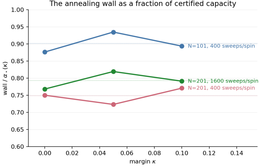
Figure 2: The annealing wall as a fraction of the certified capacity \alpha_*(\kappa) , for three size–budget pairs. Within each run the fraction is flat in \kappa to a few percent, while its level depends on both size and budget.
