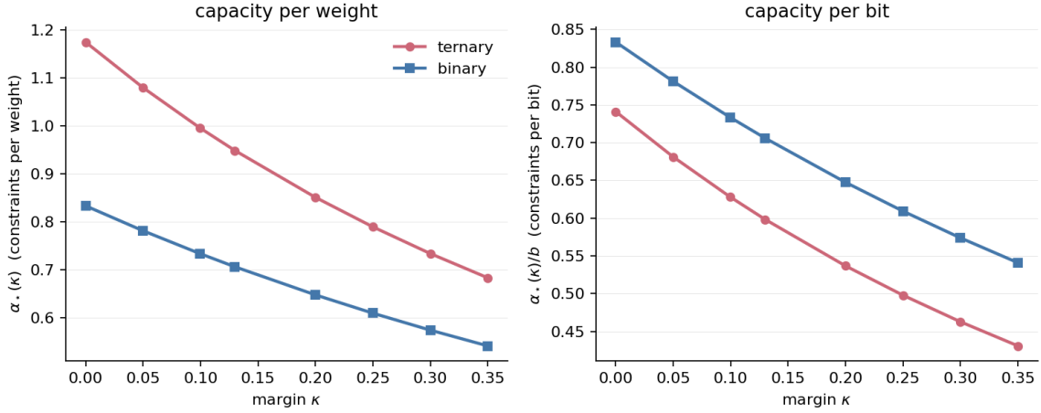
Figure 4: Replica-symmetric capacity of ternary against binary weights, per weight (left) and per stored bit (right, dividing by \log_2 3 and 1). The order reverses: the richer prior stores more per weight and less per bit, at every computed margin.
