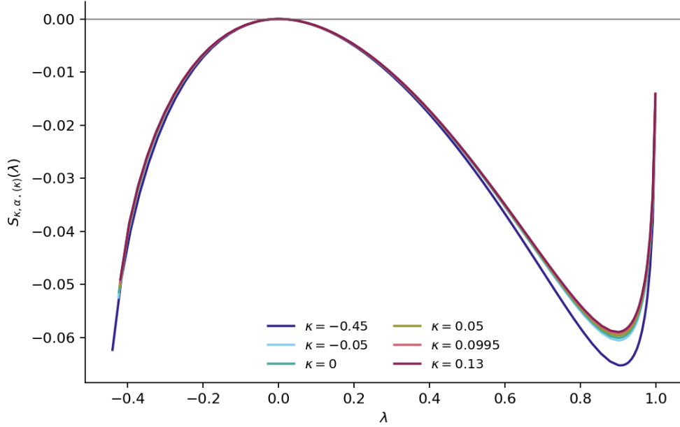
Figure 2: The general-margin Ding–Sun lower-bound condition, evaluated at the five certified margins and \kappa = 0 : the univariate function S_{\kappa, \alpha_\star(\kappa)} of their equation (48), whose nonpositivity off \{0, 1\} is the numerical hypothesis of their second-moment argument. All six curves are negative off the two roots and nearly coincide.
