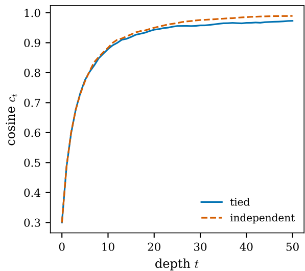
(c) ReLU angle, N=1500 : agree at fixed t
