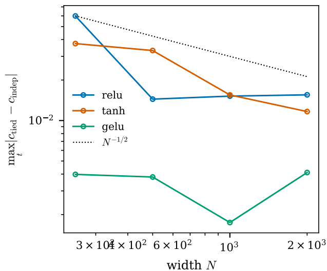
(b) agreement improves as N^{-1/2}
