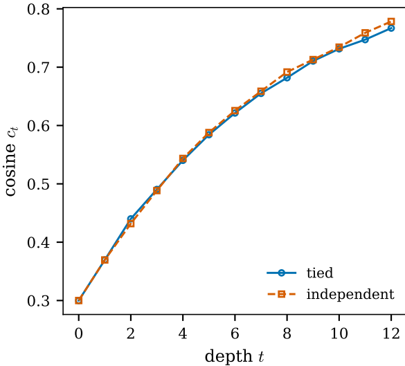
(a) tanh, N=2000 : tied = independent
