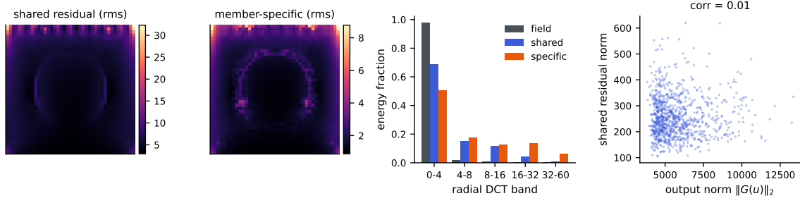
Figure S6.2: Anatomy of the shared residual c (across-member mean of the residual fields), at one seed. Left to right: rms of c over the grid; rms of the member-specific remainders; radial DCT band energies of the stress fields, of c , and of the specific parts; and the norm of c against the output norm, whose correlation is 0.01.
