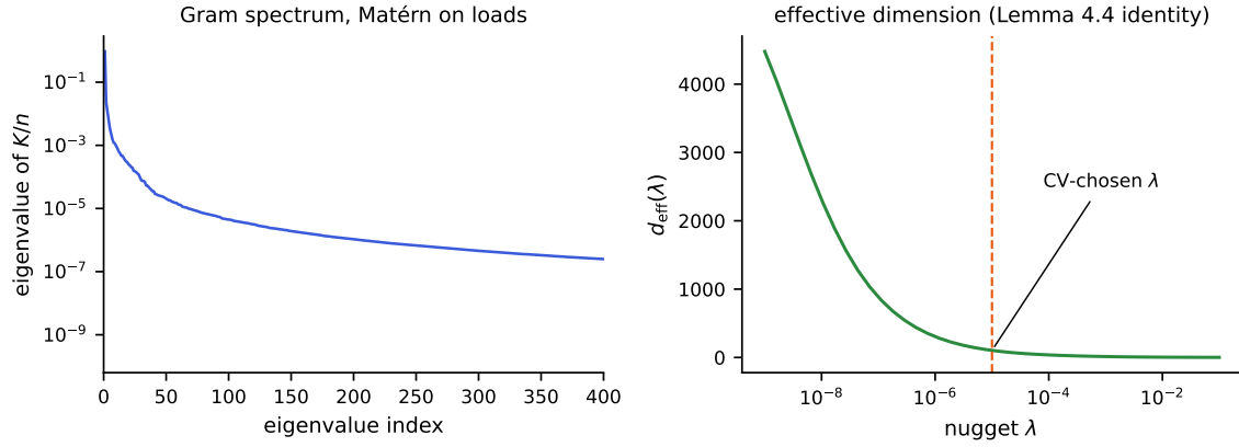
Figure S6.3: Left: eigenvalues of the Matérn Gram matrix K/n on the loads (log scale); the spectrum decays by many orders of magnitude within a few hundred modes. Right: the effective dimension d_{\text{eff}}(\lambda) from the exact identity of Lemma S5.1, with the cross-validated nugget marked.
