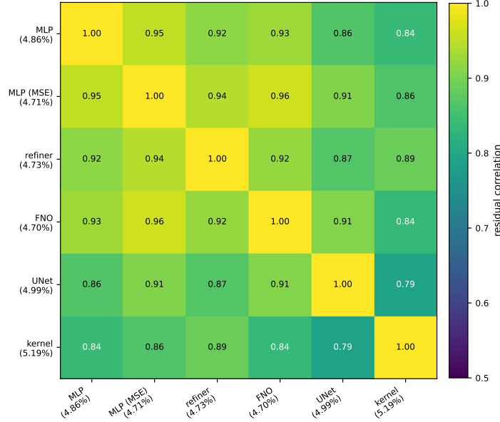
Figure S6.1: Correlation of per-sample normalized residuals on the validation split, drawn at one seed from the original single-run study, which also trained a UNet member (test-set values agree to two decimals). Across the ten replicated seeds, whose five members all appear here, every pair correlates between 0.83 and 0.97, with a mean of 0.913 \pm 0.005 ; the kernel predictor, the most alien member by construction, still correlates 0.86–0.88 with the most accurate network at every one of them.
