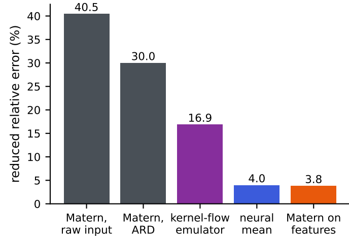
the same kernel, three feature sets (O2)
