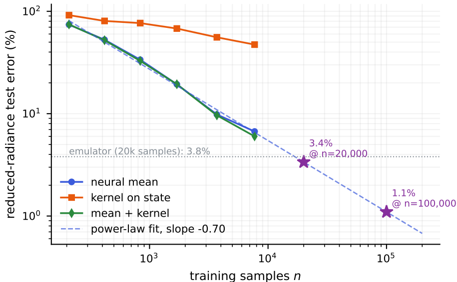
OCO-2 O 2 emulator: test error versus training-set size
