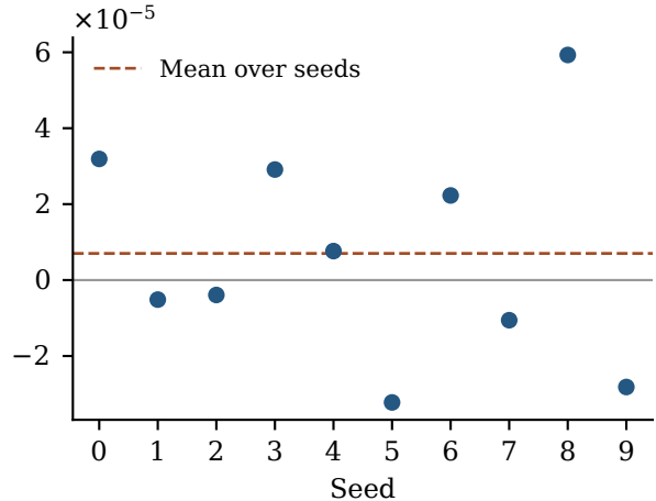
(b) Correction labels: query-time-consistent minus original
