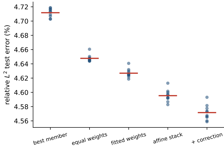
the same ten seeds, stage by stage
