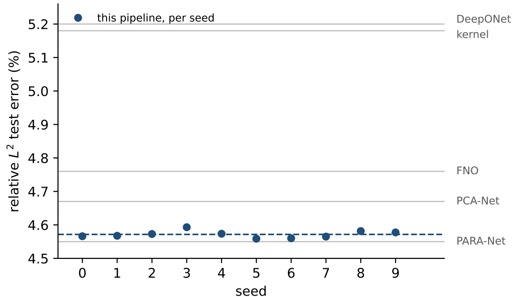
ten replicates against five published methods
