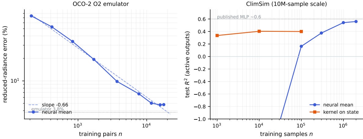
Figure 9: Test error against training-set size, at fixed test set. Left: the OCO-2 O2 emulator, reduced-radiance error; the neural mean falls as a power law (fitted slope -0.66 ) to 4.6% at n = 15700 , and the dotted line marks the published emulator’s 3.8%. Right: ClimSim, test R^2 over the outputs with non-negligible variance; the exact kernel is flat and data-efficient while the neural mean, underfit at small n , overtakes it near a few hundred thousand samples and approaches the published baseline (dotted) by two million.
