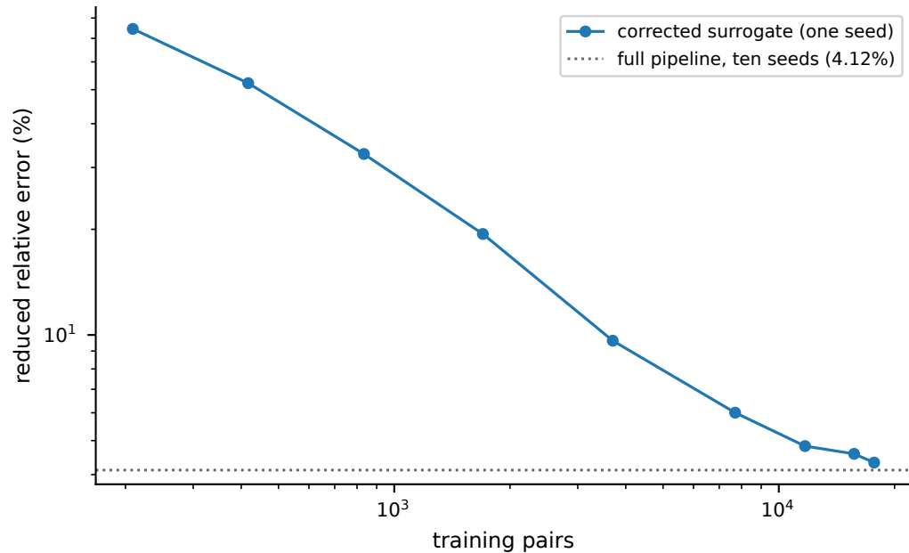
OCO-2 O2: error against training size
