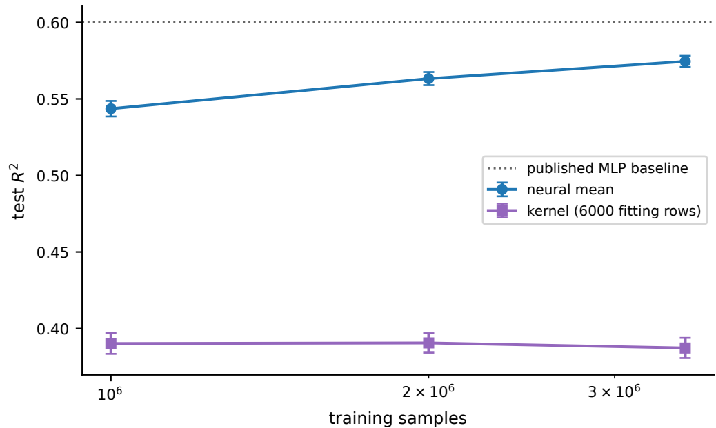
ClimSim: performance against training size
